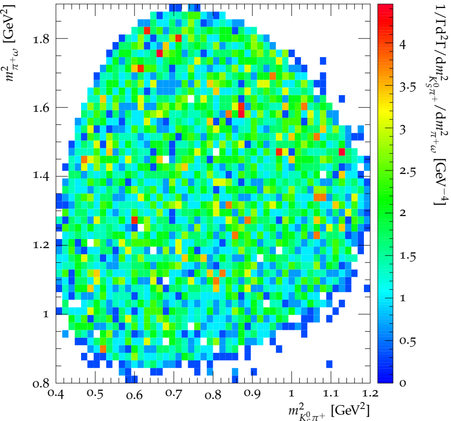
Dalitz plot for D^+ \rightarrow K_S^0 \pi^+ \omega
