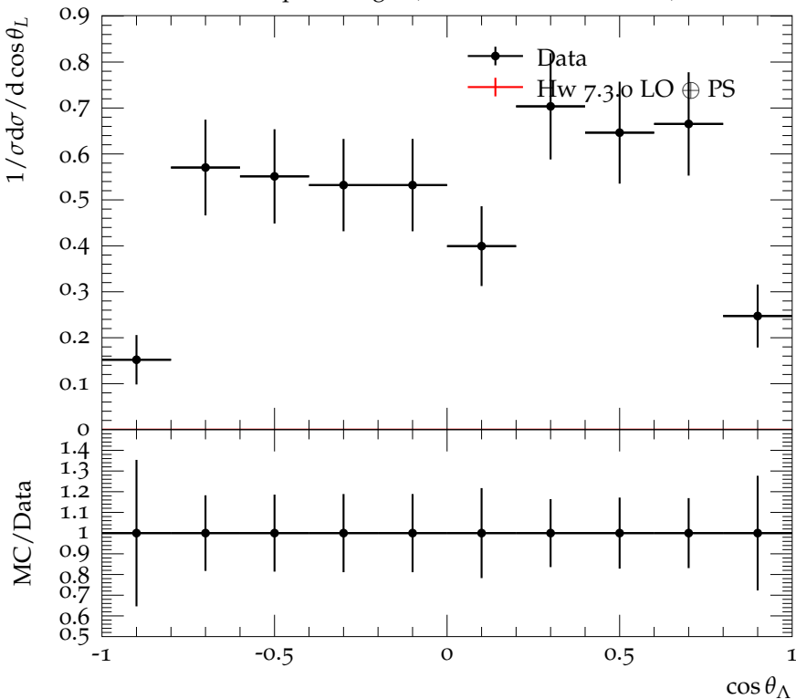
Cross section vs polar angle (N.B. data not corrected)
