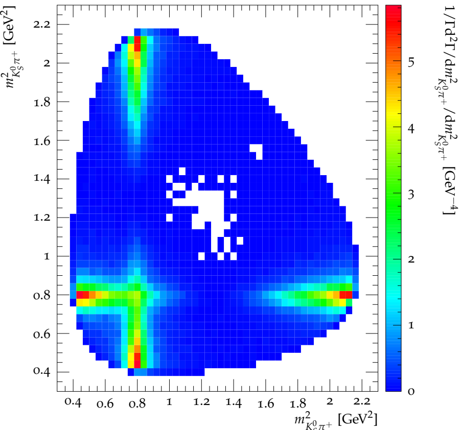
Dalitz plot for D_s^+ \rightarrow K_S^0 K_S^0 \pi^+
