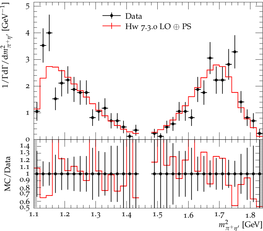
\pi^+\eta' mass distribution in D_s^+ \rightarrow \pi^+\pi^0\eta'
