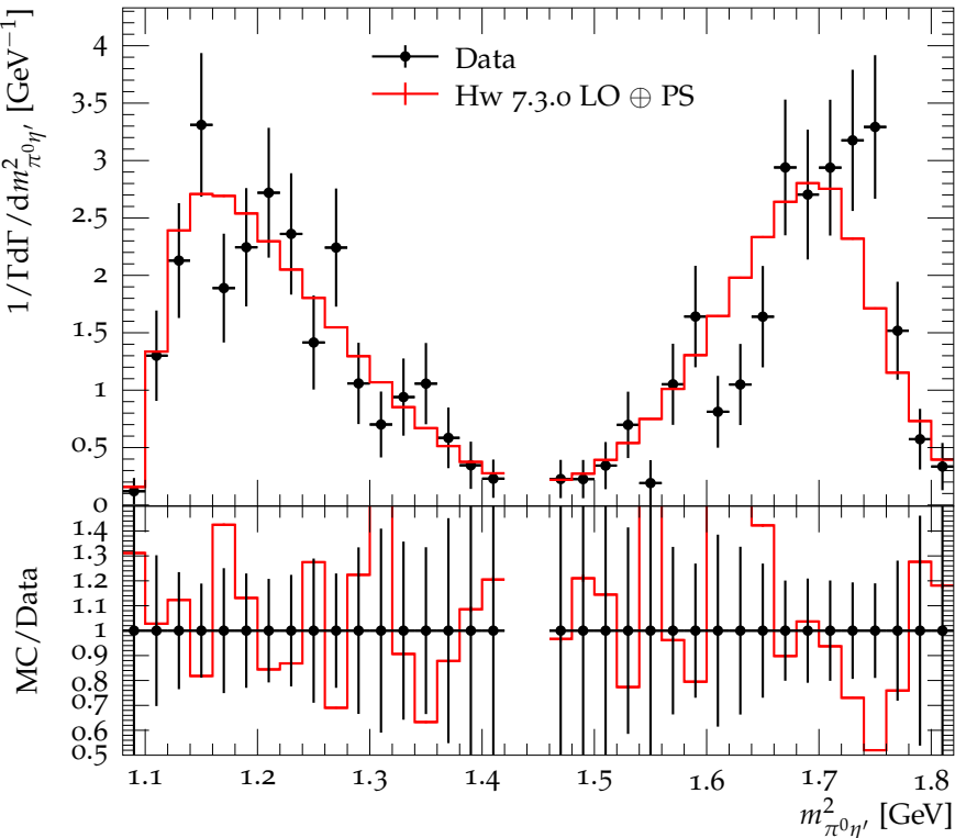
\pi^0\eta' mass distribution in D_s^+ \rightarrow \pi^+\pi^0\eta'
