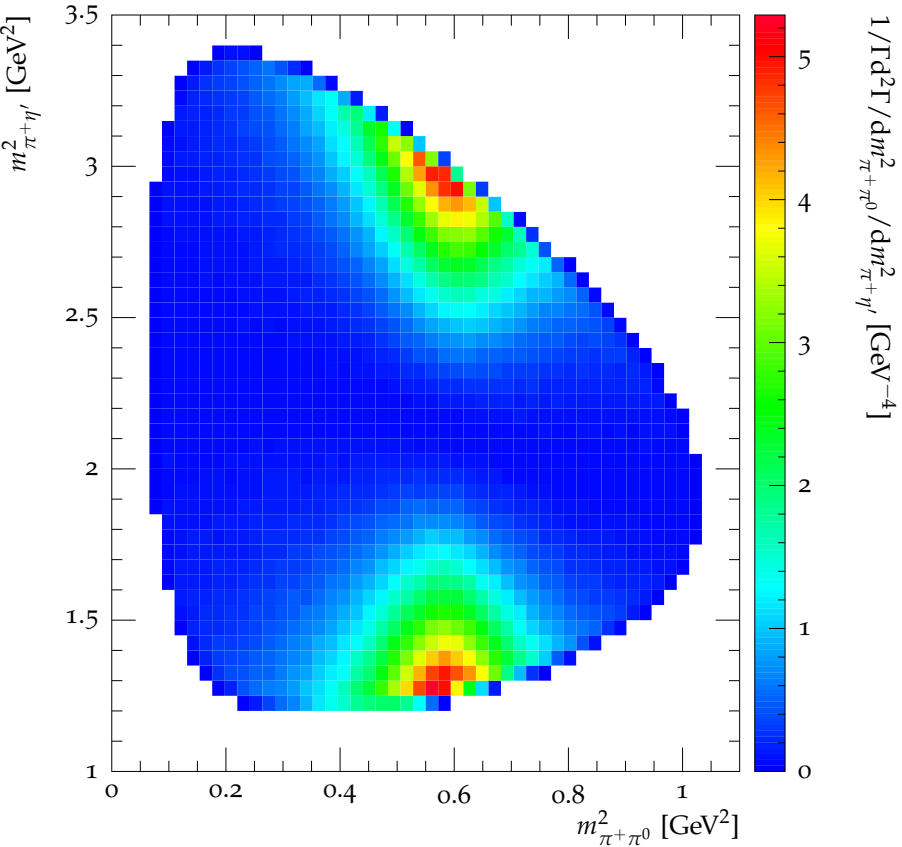
Dalitz plot for D_s^+ \rightarrow \pi^+ \pi^0 \eta'
