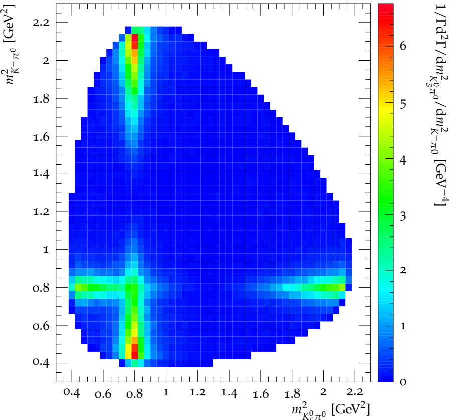
Dalitz plot for D_s^+ \rightarrow K_S^0 K^+ \pi^0
