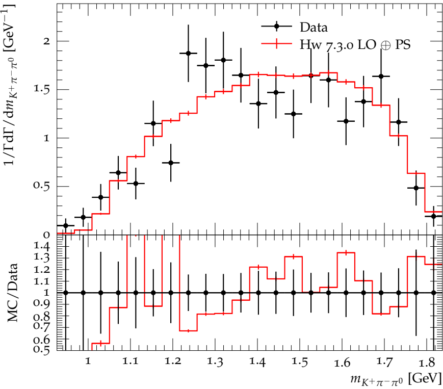
K^+ \pi^- \pi^0 mass distribution in D_s^+ \rightarrow K^+ \pi^+ \pi^- \pi^0
