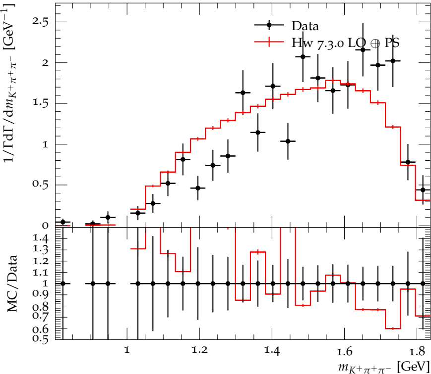
K^+ \pi^+ \pi^- mass distribution in D_s^+ \rightarrow K^+ \pi^+ \pi^- \pi^0
