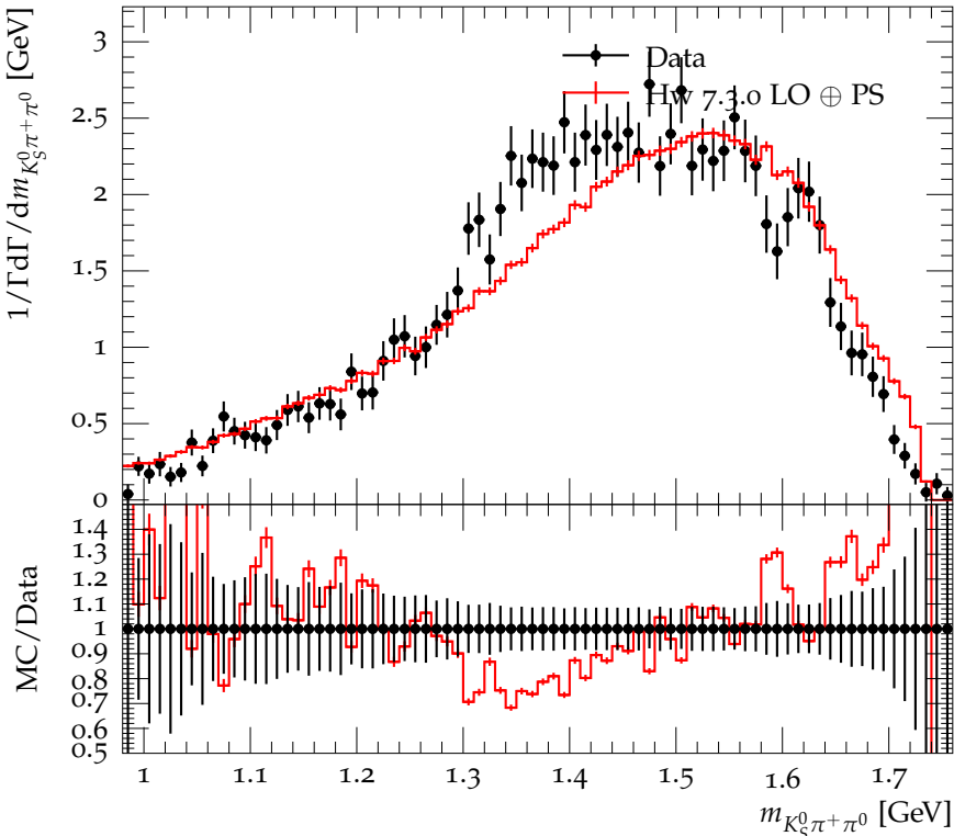
K_S^0\pi^+\pi^0 mass distribution in D^0 \rightarrow K_S^0\pi^+\pi^0\pi^0
