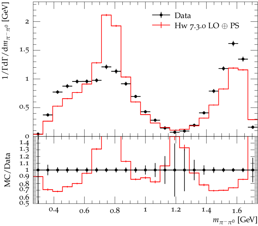
\pi^- \pi^0 mass distribution in D^0 \rightarrow \pi^+ \pi^- \pi^0
