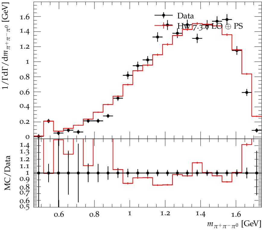
\pi^+\pi^-\pi^0 mass distribution in D^0 \rightarrow \pi^+\pi^-\pi^0
