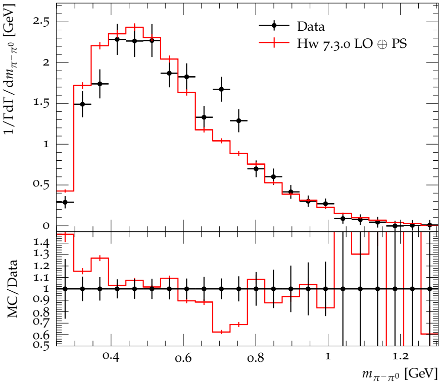
\pi^- \pi^0 mass distribution in D^0 \rightarrow 2\pi^+ 2\pi^- \pi^0
