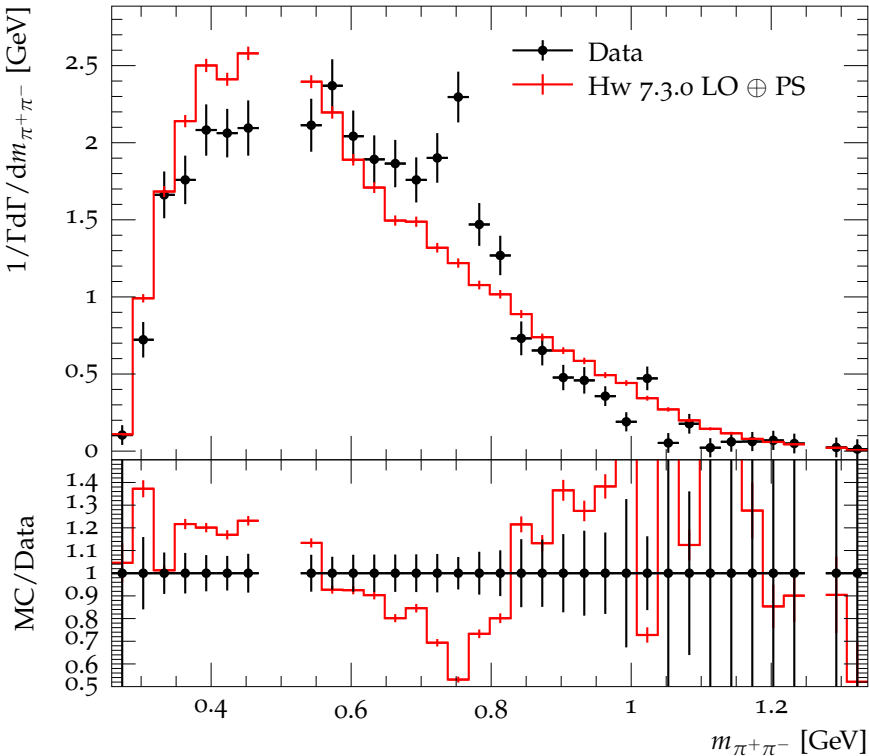
\pi^+\pi^- mass distribution in D^0 \rightarrow 2\pi^+2\pi^-\pi^0
