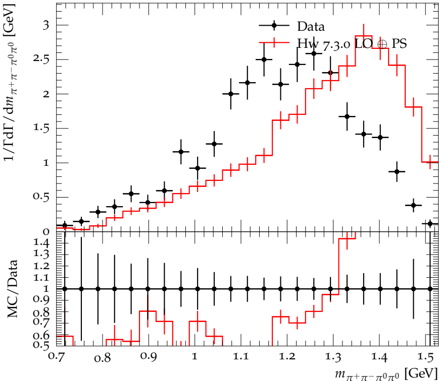
\pi^+\pi^-\pi^0\pi^0 mass distribution in D^0 \rightarrow 2\pi^+2\pi^-2\pi^0
