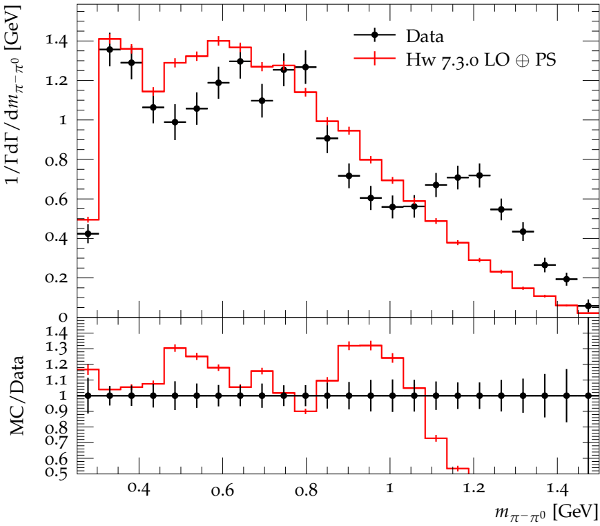
\pi^- \pi^0 mass distribution in D^+ \rightarrow 2\pi^+ \pi^- \pi^0
