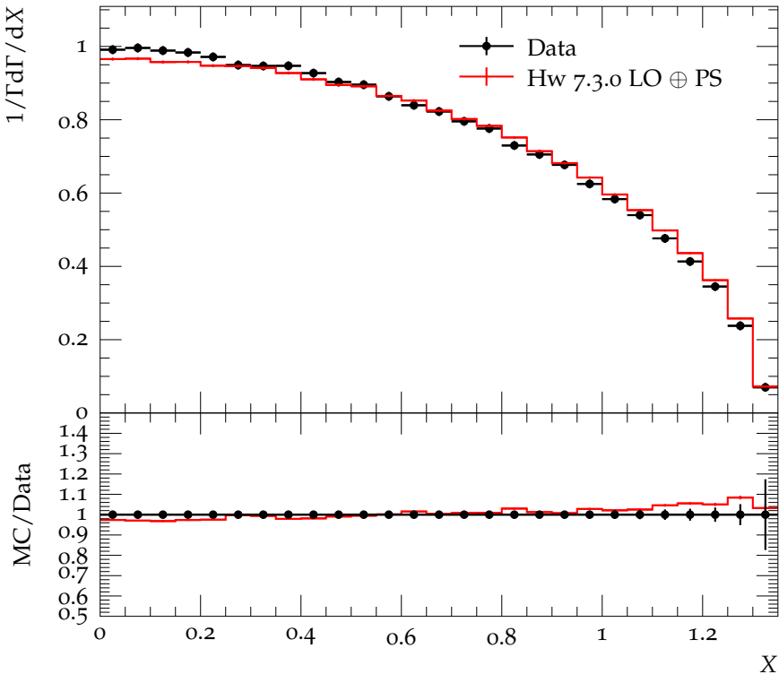
X distribution for \eta' \rightarrow \eta\pi^0\pi^0
