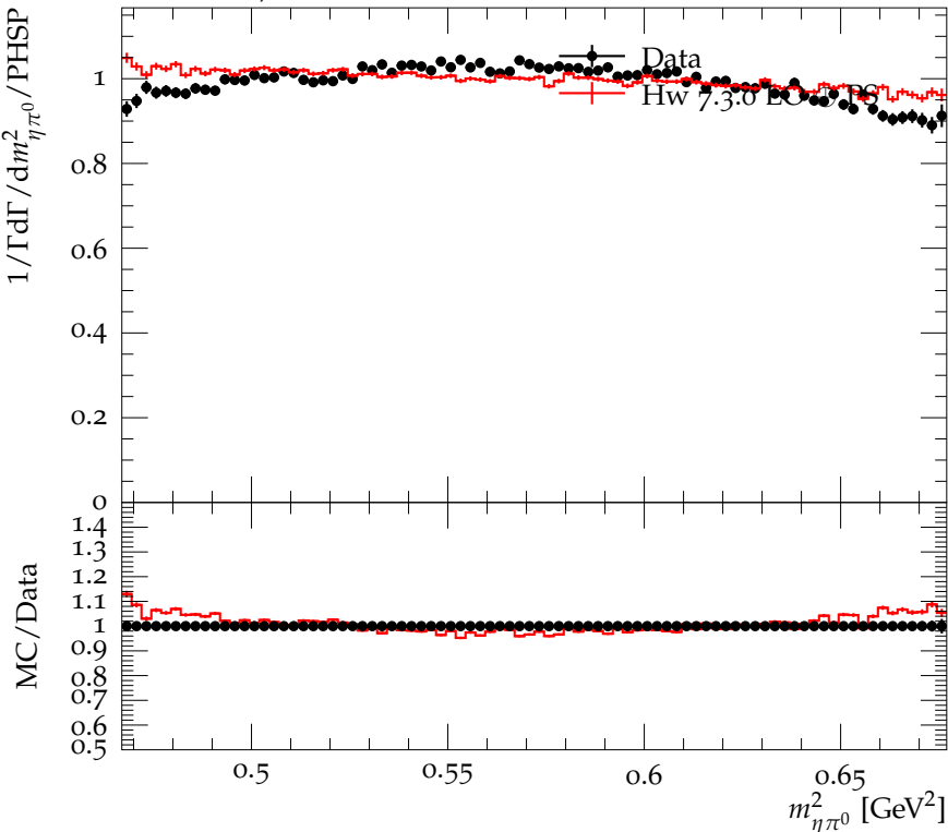
Ratio of m^2_{\eta\pi^0} distribution to phase-space for \eta' \rightarrow \eta\pi^0\pi^0
