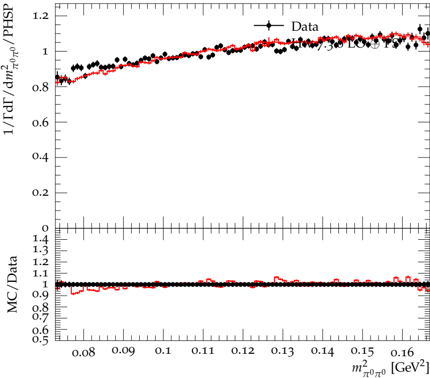
Ratio of m_{\pi^0\pi^0}^2 distribution to phase-space for \eta' \rightarrow \eta\pi^0\pi^0
