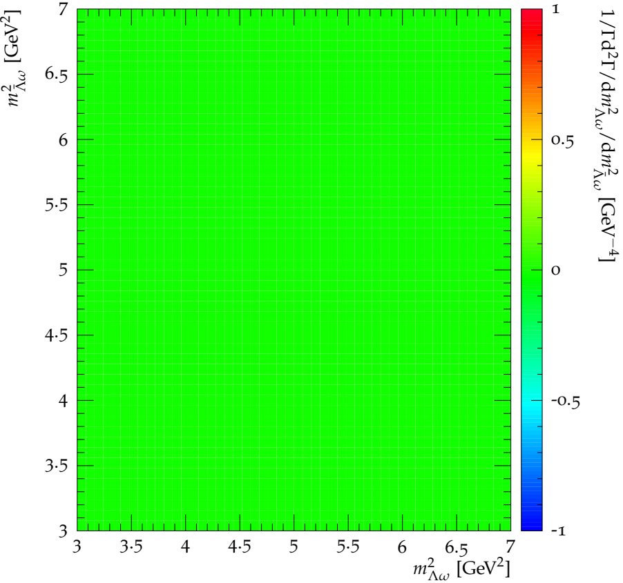
Dalitz plot for \psi(2S) \rightarrow \Lambda \bar{\Lambda} \omega
