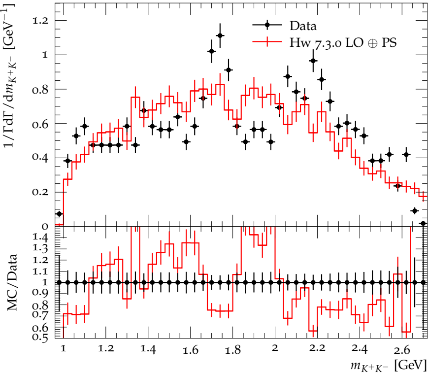
K^+K^- mass distribution in \chi_{c0} \rightarrow \pi^+\pi^-K^+K^-
