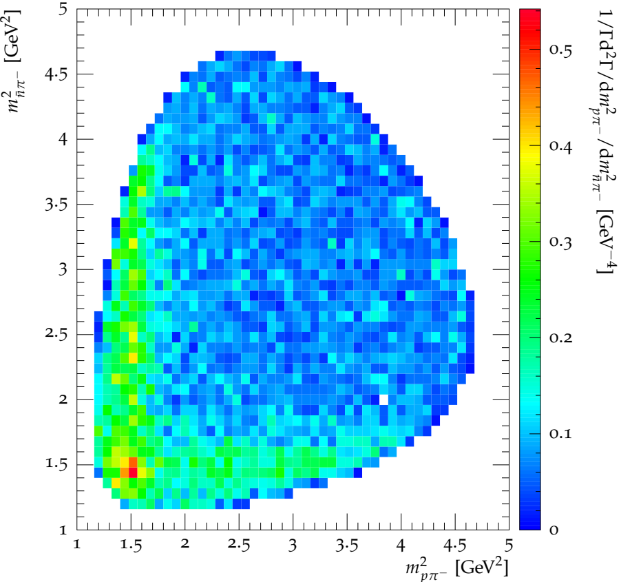
Dalitz plot for J/\psi \rightarrow p\bar{n}\pi^-
