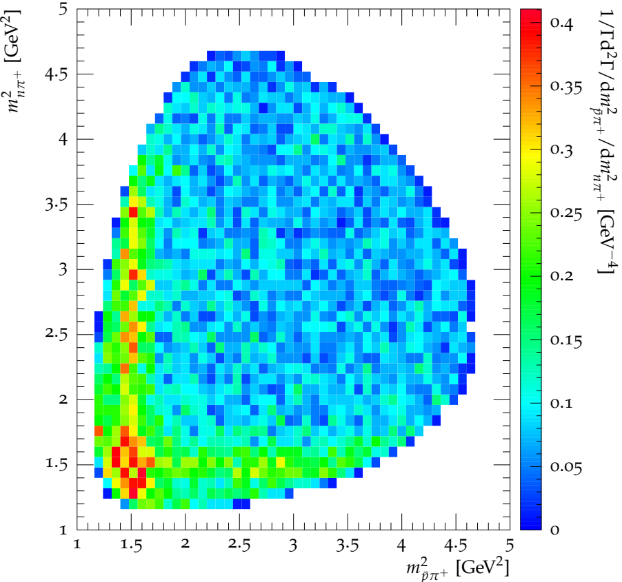
Dalitz plot for J/\psi \rightarrow n\bar{p}\pi^+
