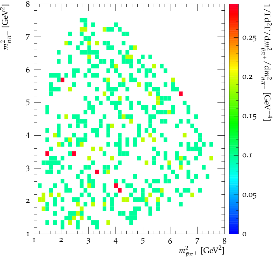
Dalitz plot for \psi(2S) \rightarrow n\bar{p}\pi^+
