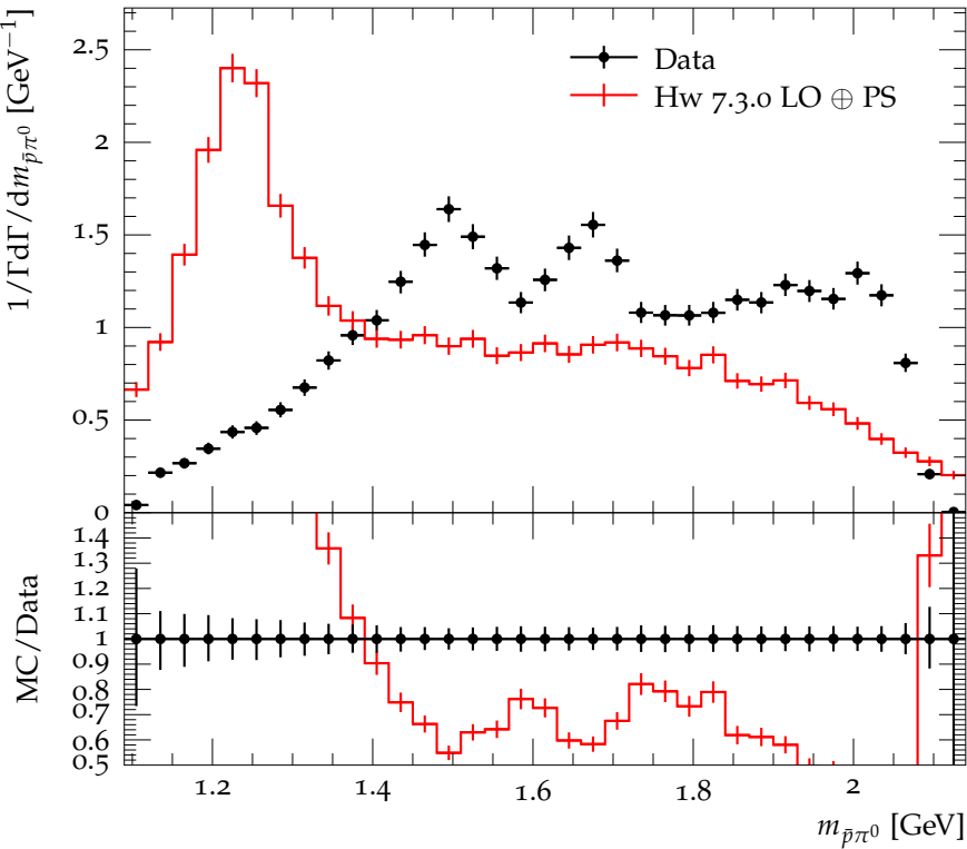
\bar{p}\pi^0 mass distribution in J/\psi \rightarrow p\bar{p}\pi^0
