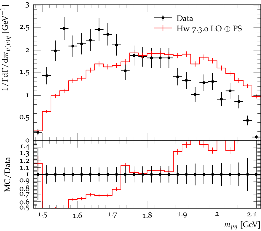
p(\bar{p})\eta mass distribution in J/\psi \rightarrow p\bar{p}\eta
