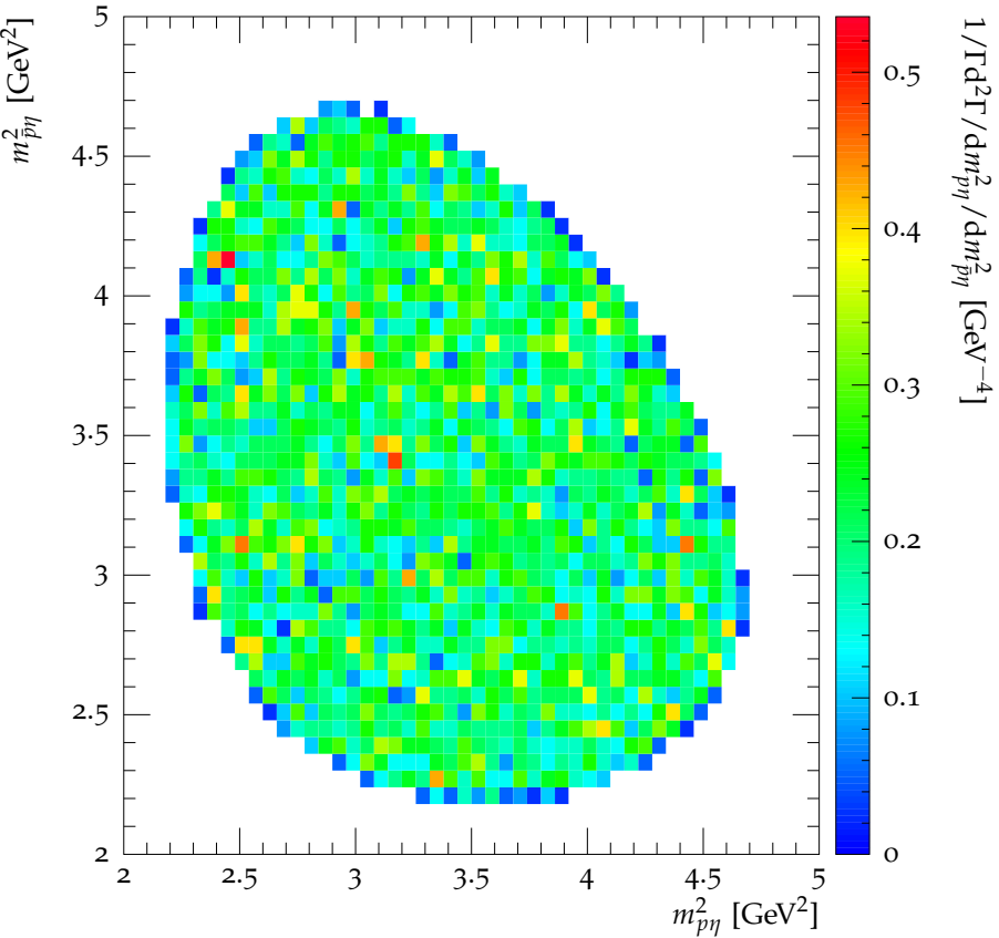
Dalitz plot for J/\psi \rightarrow p\bar{p}\eta
