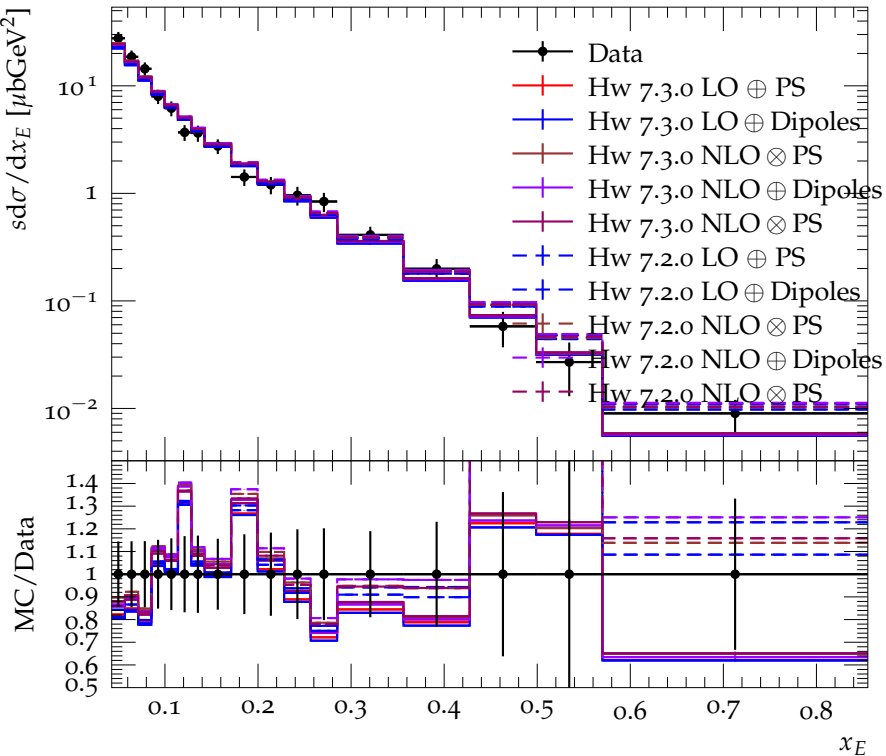
Photon spectrum at E_{\text{CMS}} = 14 \text{ GeV}
