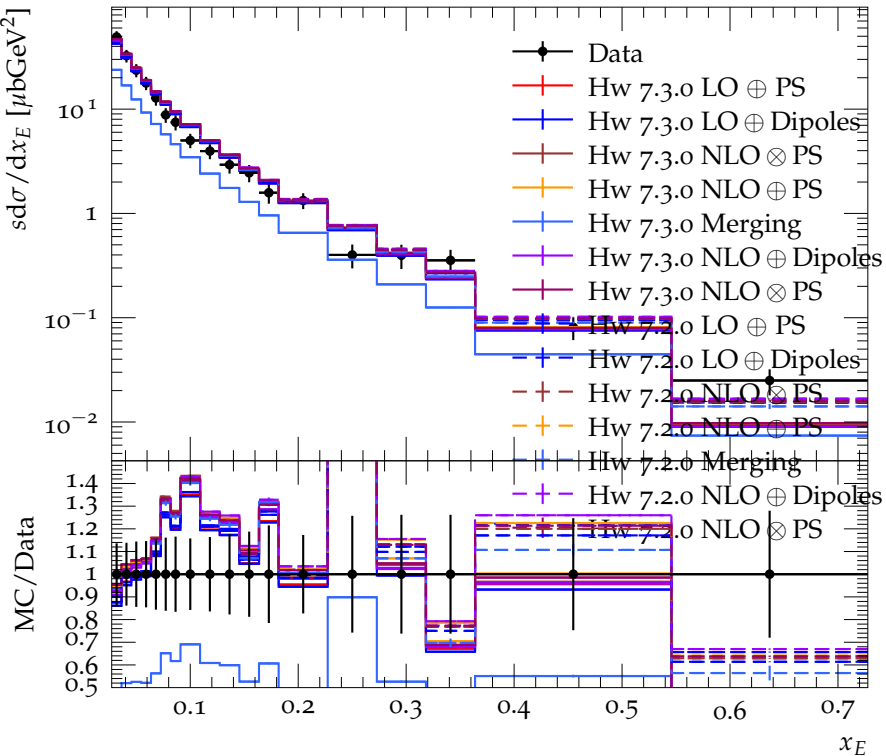
Photon spectrum at E_{\text{CMS}} = 22 GeV
