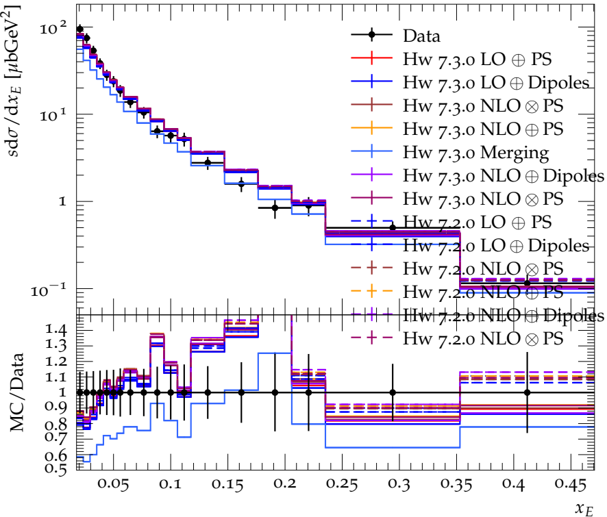
Photon spectrum at E_{\text{CMS}} = 34 \text{ GeV}
