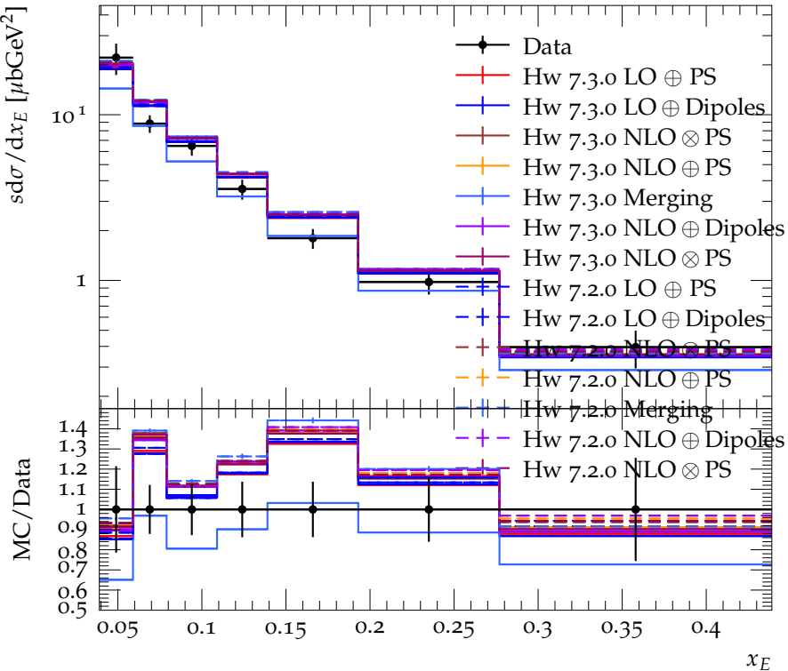
\pi^0 spectrum at E_{\text{CMS}} = 35 GeV
