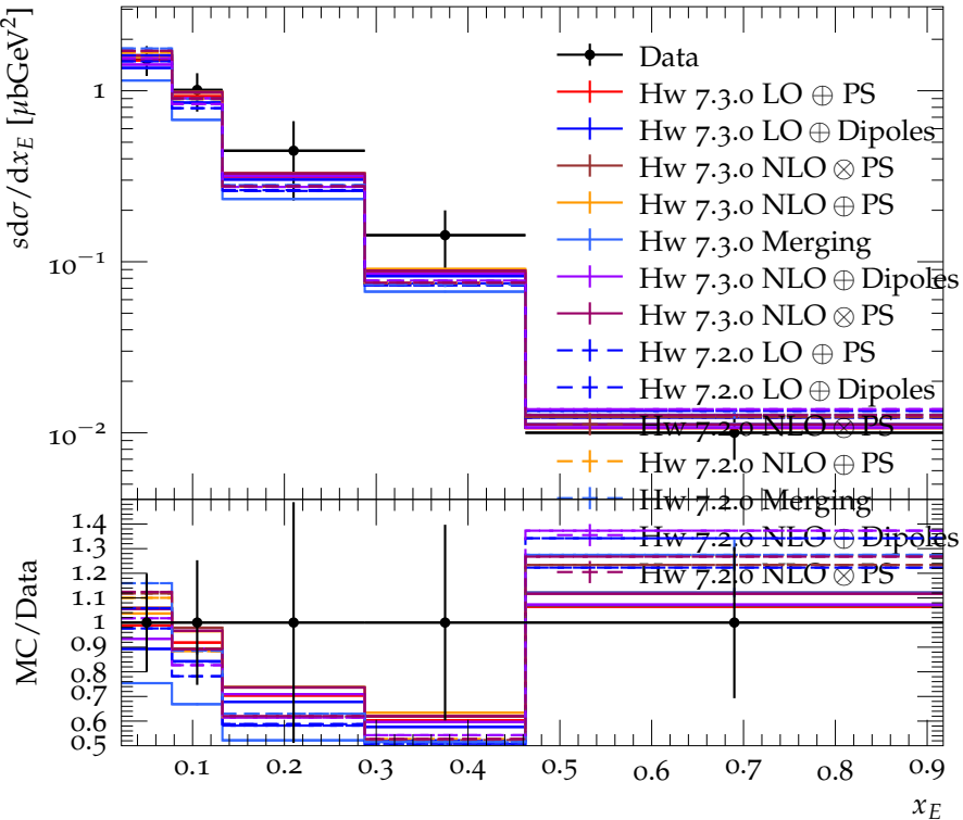
\eta spectrum at E_{\text{CMS}} = 35 GeV
