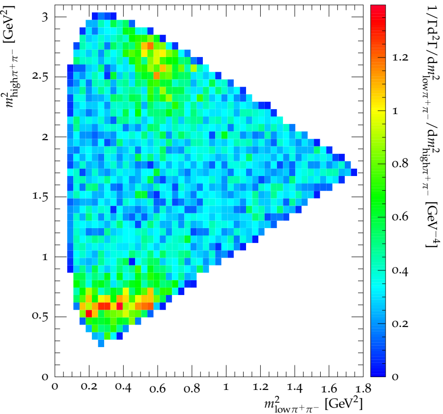
Dalitz plot for D^+ \rightarrow \pi^+ \pi^+ \pi^-
