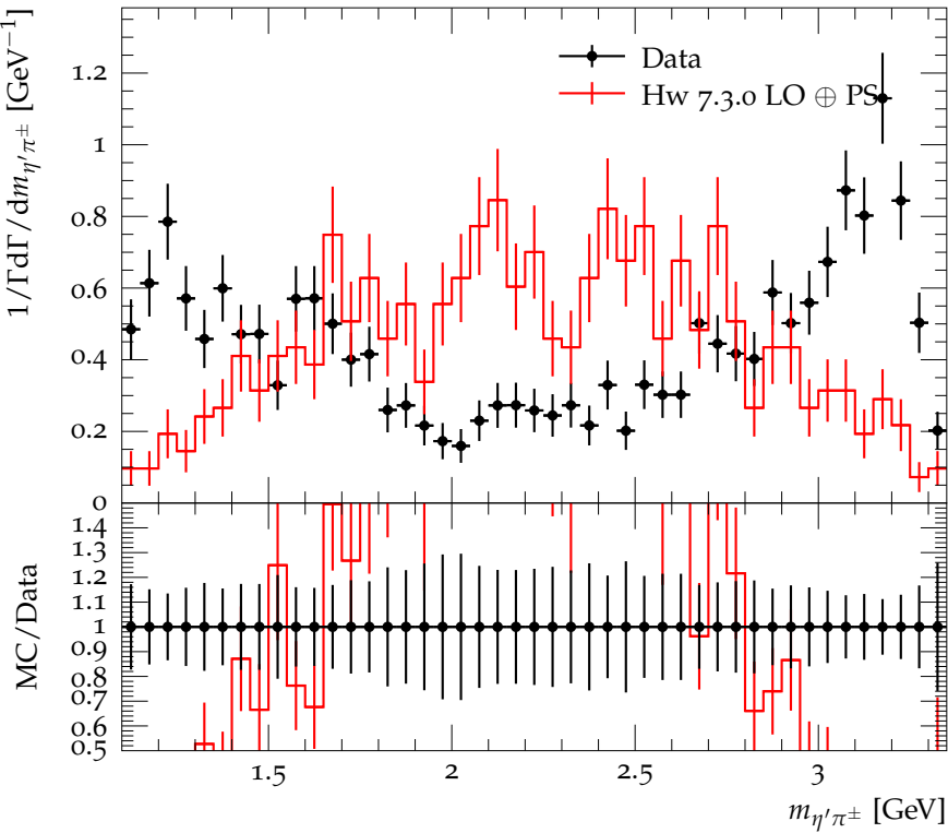
\eta' \pi^\pm mass distribution in \chi_{c1} \rightarrow \eta' \pi^+ \pi^-
