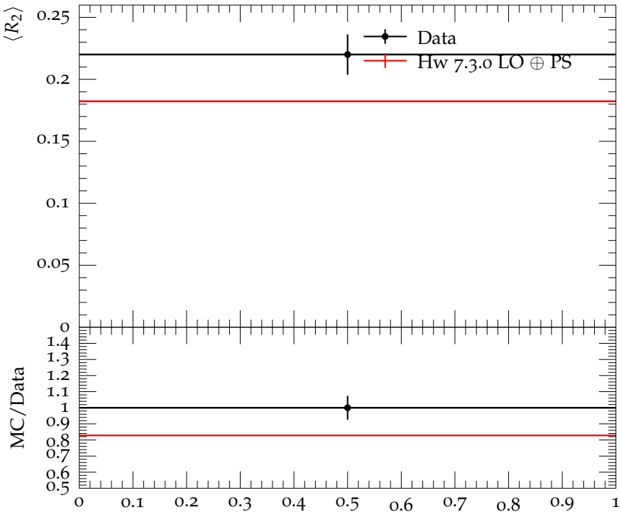
Average 2nd Fox-Wolfram momentum in \chi_{b2}(2S) decays
