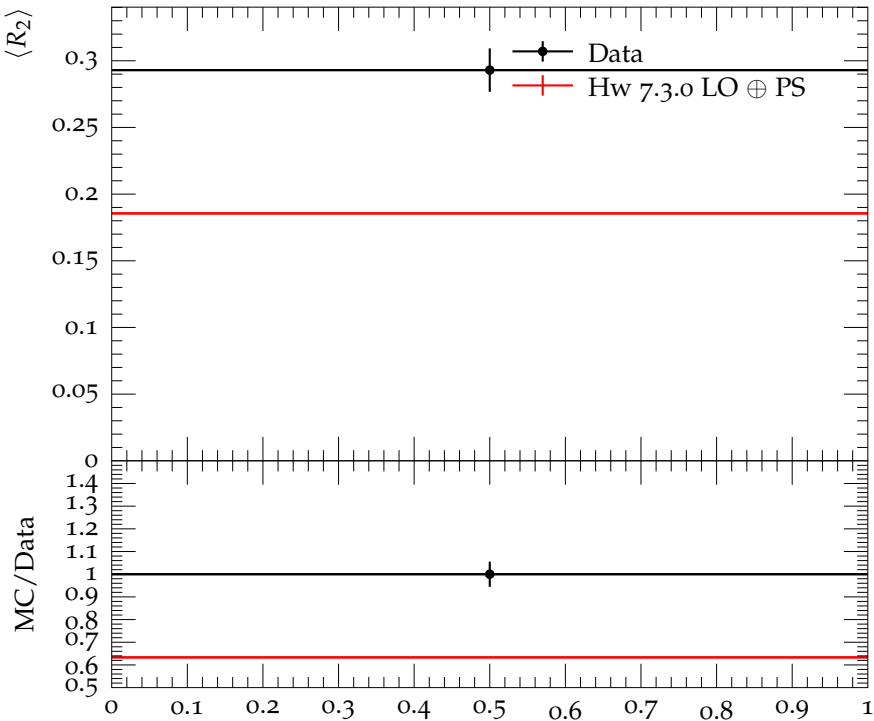
Average 2nd Fox-Wolfram momentum in \chi_{b1}(2S) decays
