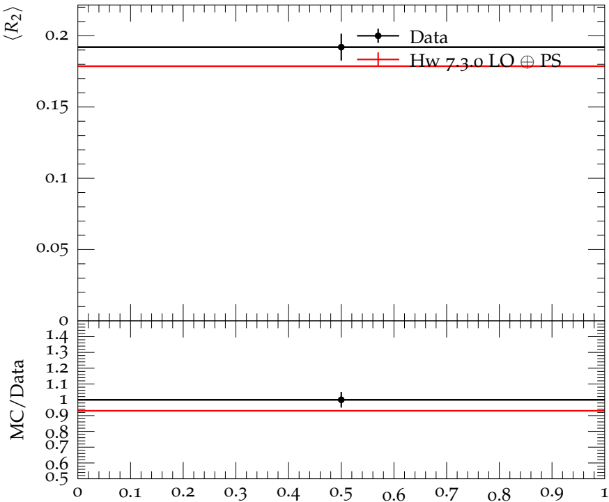
Average 2nd Fox-Wolfram momentum in \chi_{b0}(2S) decays
