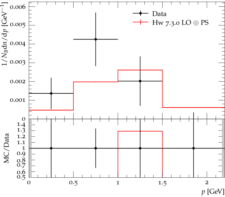
Momentum spectrum for \Sigma_c^{++}
