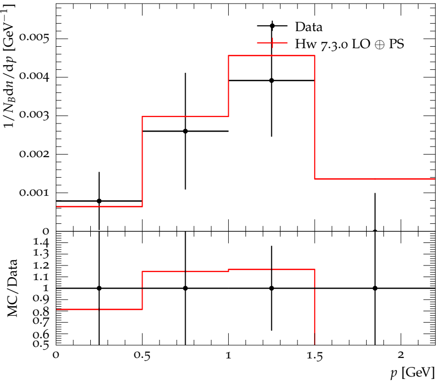
Momentum spectrum for \Sigma_c^0
