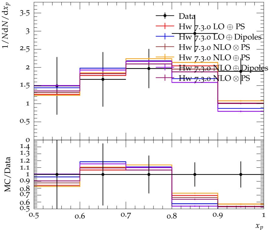
Scaled momentum spectrum for D_1(2420)^0 production
