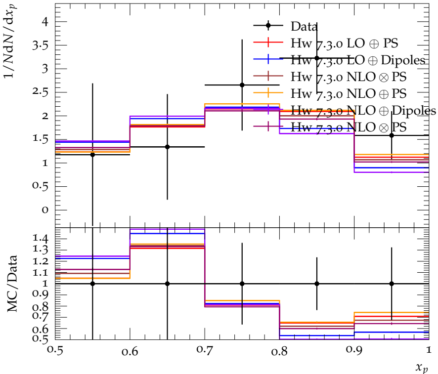
Scaled momentum spectrum for D_2(2460)^+ production
