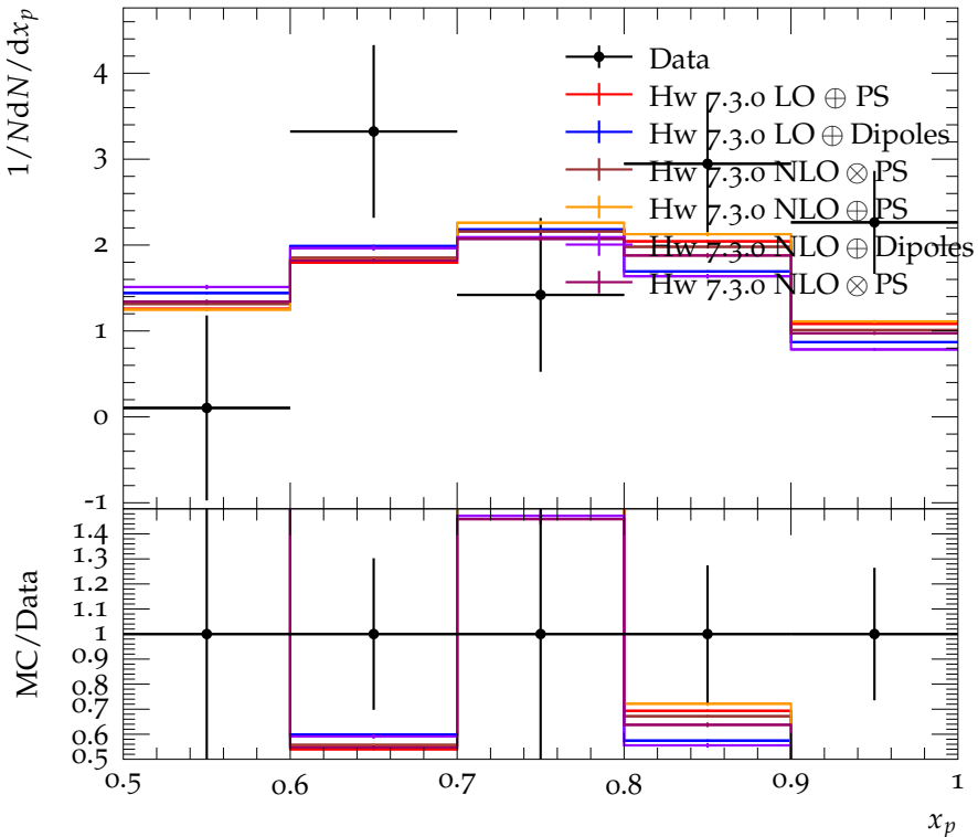
Scaled momentum spectrum for D_1(2420)^+ production
