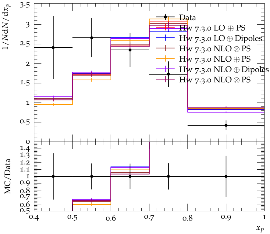
Spectrum for \Sigma_c^*
