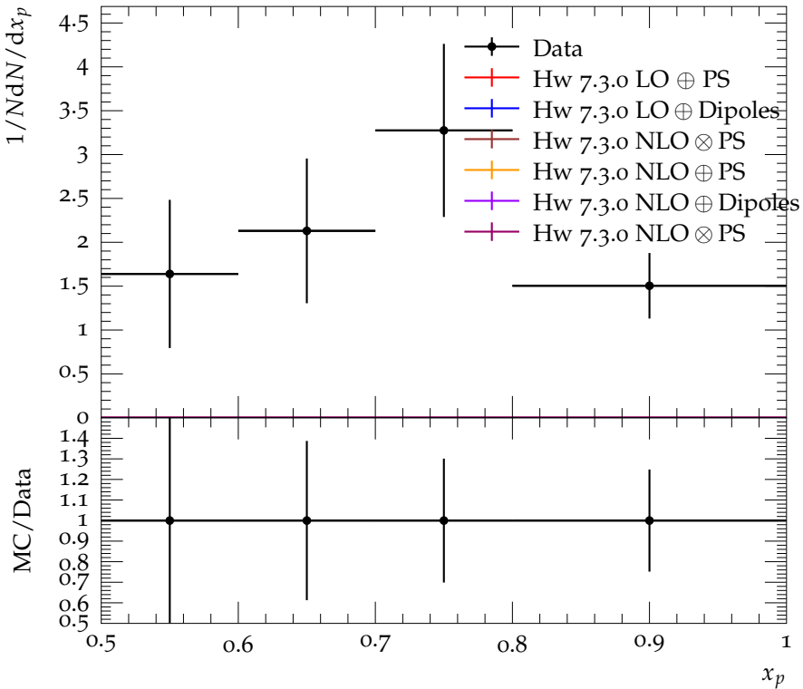
Spectrum for \Xi_c(2815)
