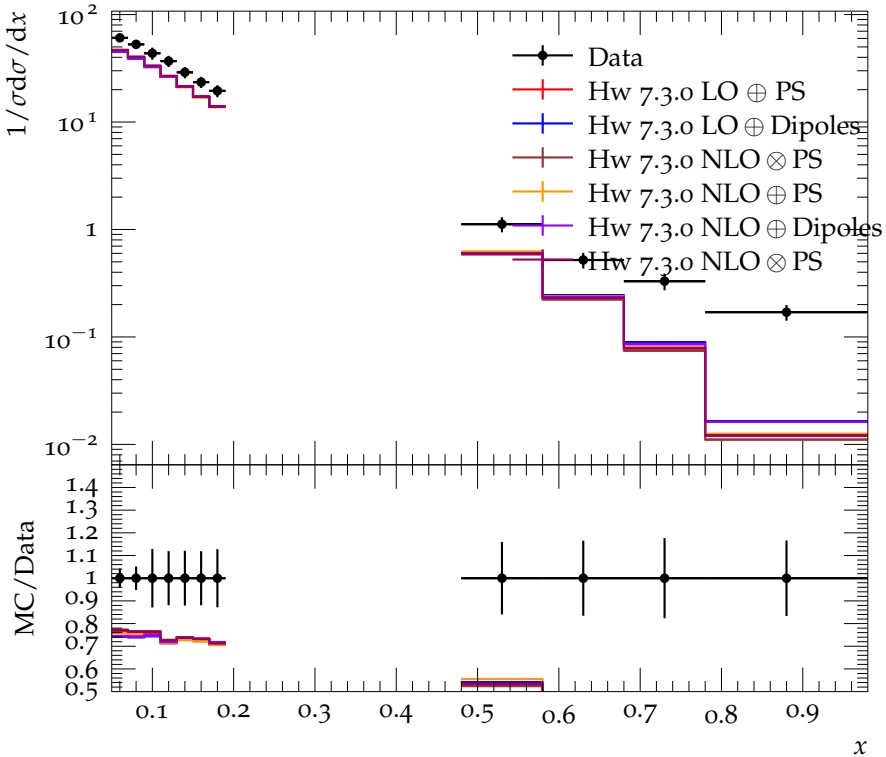
Scaled momentum spectrum for \pi^\pm in the continuum
