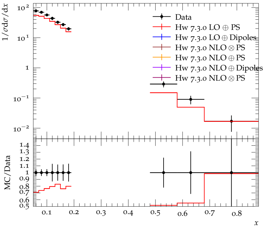
Scaled momentum spectrum for \pi^\pm at the Y(1S)
