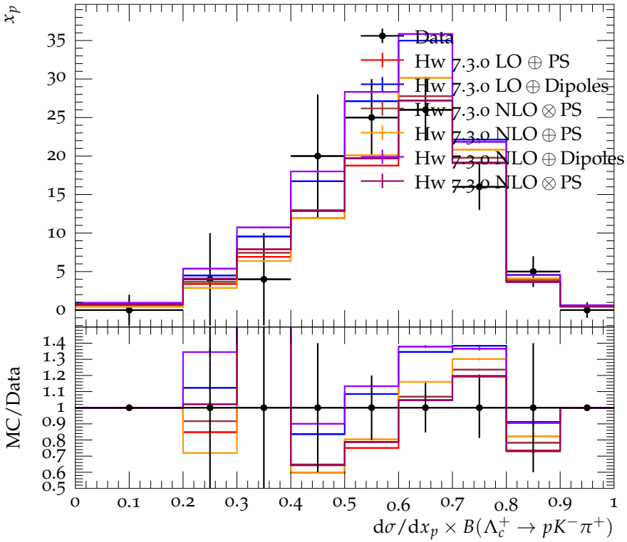
Scaled momentum spectrum for \Lambda_c^+ \rightarrow pK^- \pi^+
