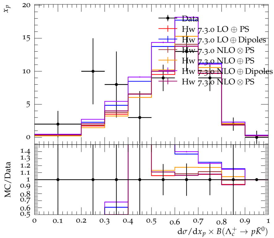
Scaled momentum spectrum for \Lambda_c^+ \rightarrow p\bar{K}^0
