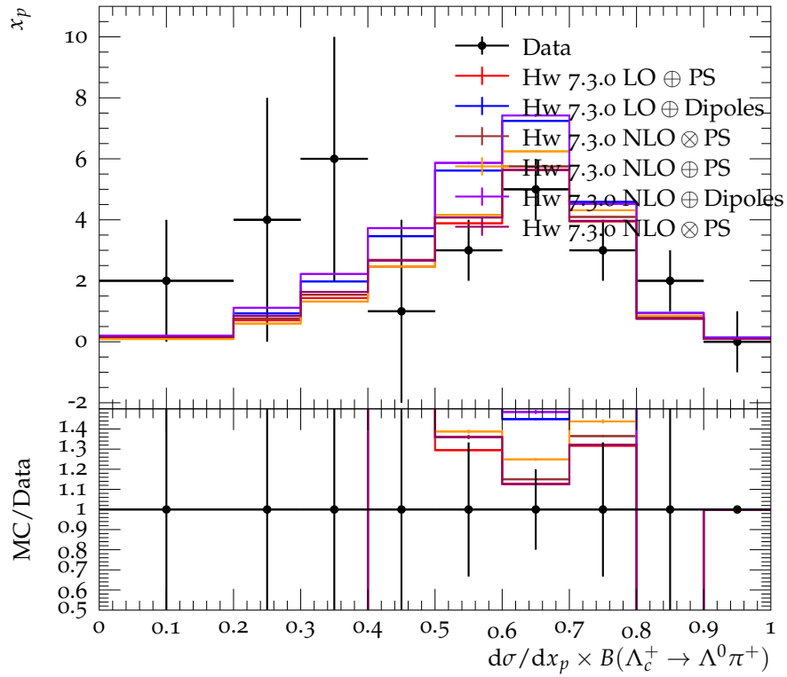
Scaled momentum spectrum for \Lambda_c^+ \rightarrow \Lambda^0 \pi^+
