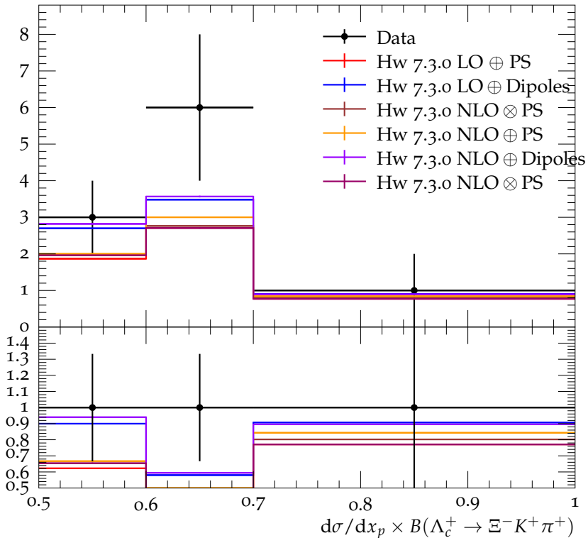
Scaled momentum spectrum for \Lambda_c^+ \rightarrow \Xi^- K^+ \pi^+
